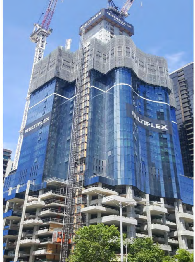
108 Storey Tower - Melbourne Australia
